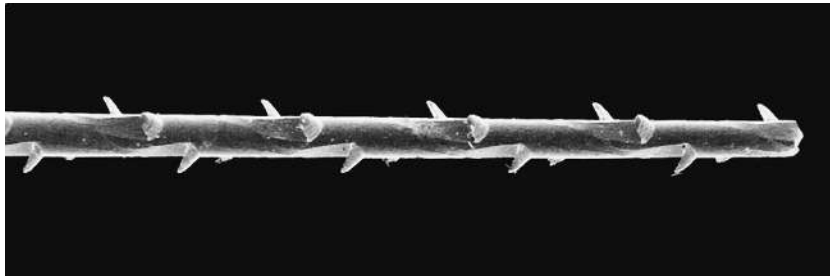
Fig. 8.23 Scanning electron micrograph of a barbed broach. (Courtesy Moyco Union Broach, York, PA, USA.)
