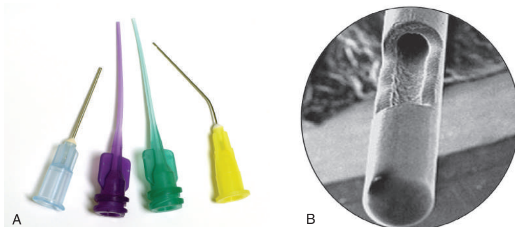
Fig. 8.46. A, Various types of needles for root canal irrigation. Shown are examples with open end and closed end, side vented. These are manufactured from plastic and stainless steel. B, SEM image of 30 gauge safety needle. (Courtesy Dr. F. Tay.)
