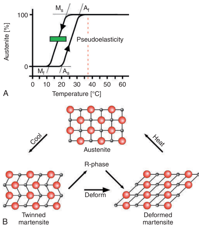
Fig. 8.19 Pseudoelastic behavior of nickel titanium is based on the two main crystal configurations, martensite and austenite, which depend on temperature (A) and applied strain (B). Formation of the respective configuration initiates at the start temperatures, M_s and A_s .
