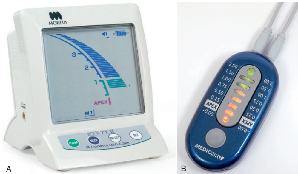
Fig. 8.36 Root ZX apex locator with lip clip and file holder. (A, Courtesy J. Morita USA, Irvine, CA, USA). NRG miniature electronic apex locator. (B, Courtesy MedicNRG, Kibutz Afikim, Israel)
