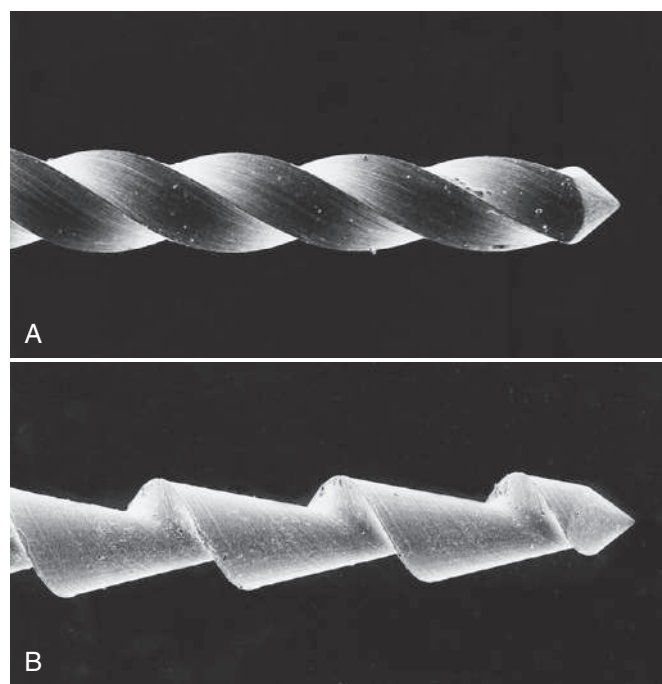
Fig. 8.17 Scanning electron micrographs of endodontic hand files fabricated by twisting (K-file size #40, A ) and grinding (Hedström file #50, B ). ( A–B , Courtesy Dentsply Maillefer, Ballaigues, Switzerland.)
