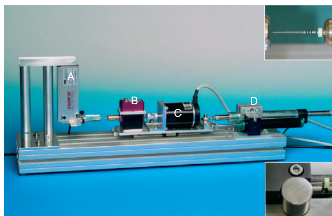
Fig. 8.63 Testing platform for analysis of various factors during simulated canal preparation with rotary endodontic instruments. Labeled components are a force transducer (A), a torque sensor (B), a direct-drive motor (C), and an automated feed device (D). For specific tests, a cyclic fatigue phantom or a brass mount compliant with ISO No. 3630-1 (inserts) may be attached.
