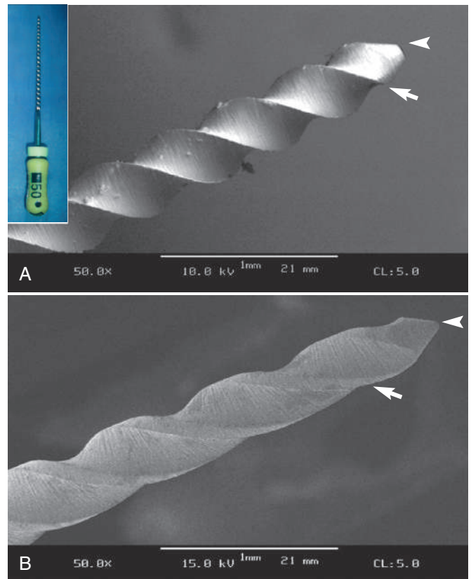
Fig. 8.12 Comparison of the flute geometry and tip configuration of a hand file ( insert ) and a NiTi rotary instrument. A , K-file with sharp cutting edges ( arrow ) and Batt tip ( arrowhead ). B , GT rotary file with rounded, noncutting tip ( arrowhead ), smooth transition, and guiding radial lands ( arrow ).
