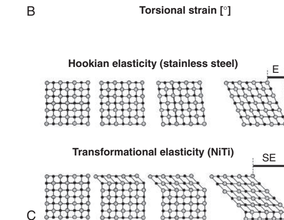
Fig. 8.18 Stress-strain behavior of nickel-titanium alloy. A , Schematic diagram of linear extension of a NiTi wire. B , Torque to failure test of a size #60, .04 taper ProFile NiTi instrument. Note the biphasic deformation, indicated by arrows in A–B . C , Comparison of stainless steel and nickel-titanium crystal lattices under load. Hookian elasticity accounts for the elastic behavior ( E ) of steel, whereas transformation from martensite to austenite and back occurs during the pseudoelastic ( PE ) behavior of NiTi alloy. ( C , Modified from Thompson SA: An overview of nickel-titanium alloys used in dentistry, Int Endod J 33:297–310, 2000.)
