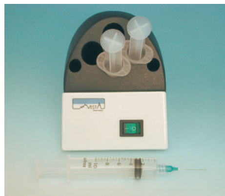
Fig. 8.49 Device for heating syringes filled with irrigation solution (e.g., sodium hypochlorite) before use. (Courtesy Vista Dental Products, Racine, WI.)
