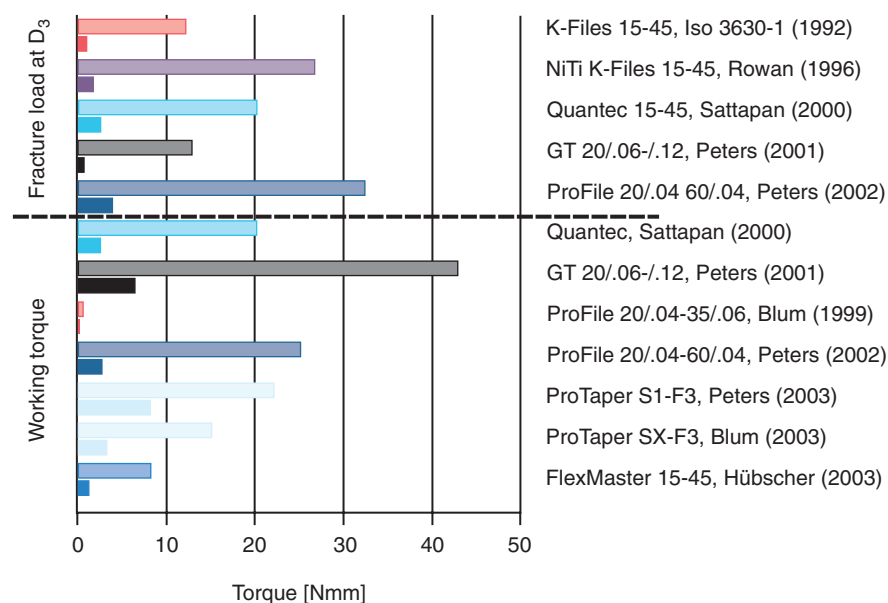
Fig. 8.31 Diagram comparing fracture loads at D_3 (upper section of graph) to torques occurring during preparation of root canals (lower section of graph). Filled columns represent the largest file in each set, and open columns show the scores of the most fragile file (see text and Box 8.3 for details).
